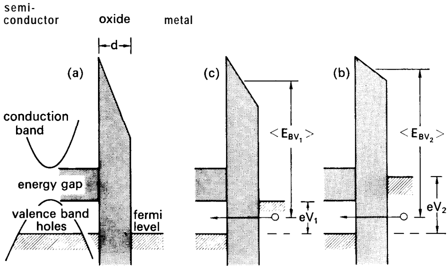
Fig. 8. Energy diagrams at varying bias-conditions in Al-Al 2 O 3 /SnTe or-GeTe tunnel junctions.
